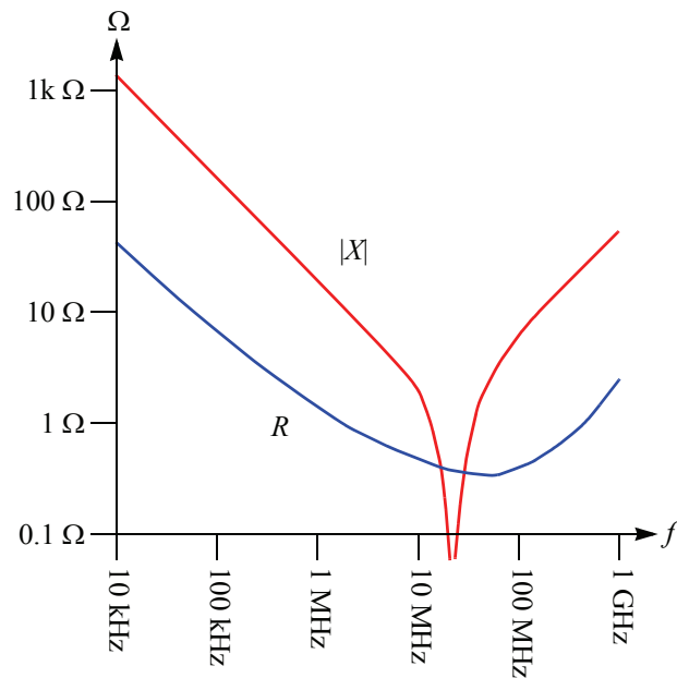
FIGURE 2. Resistance ( R ) and reactance ( X ) of a 10 nF ceramic capacitor.
