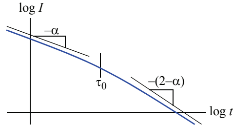
FIGURE 10. Absorptive capacitor discharge current.
